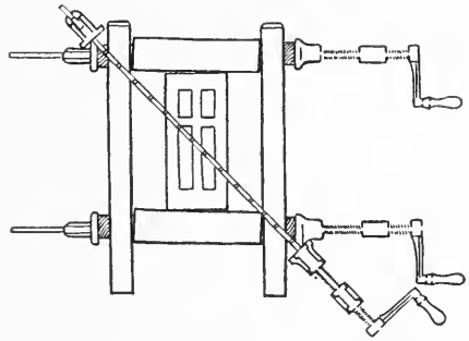
FIG. 417. DIAGONAL CLAMPING.
